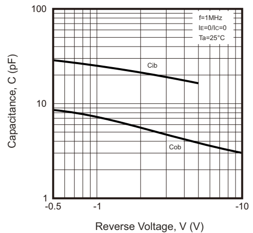
Fig.6 - C_{ob}/C_{ib} - V_{CB}/V_{EB}
